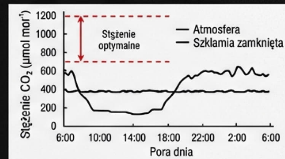
DATA REFERENCE: CO2 CONCENTRATION.
